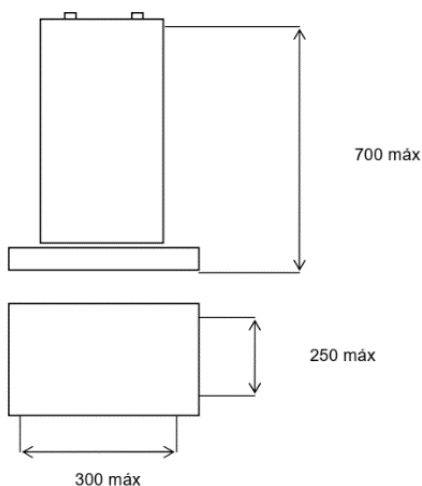
Figure 4ES (55-66 kV Indoor)
