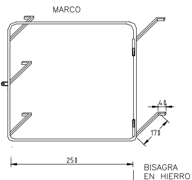
VISTA FRONTAL
