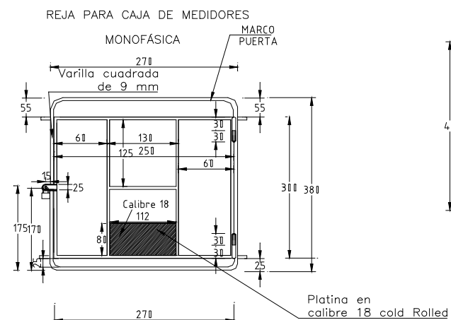
VISTA FRONTAL
