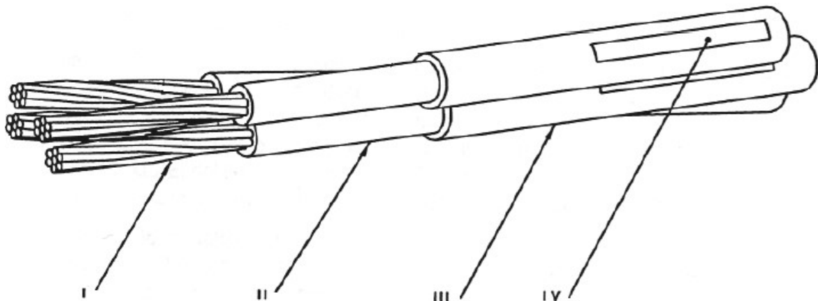
Figure 2 Schematic drawing of Type II cable
