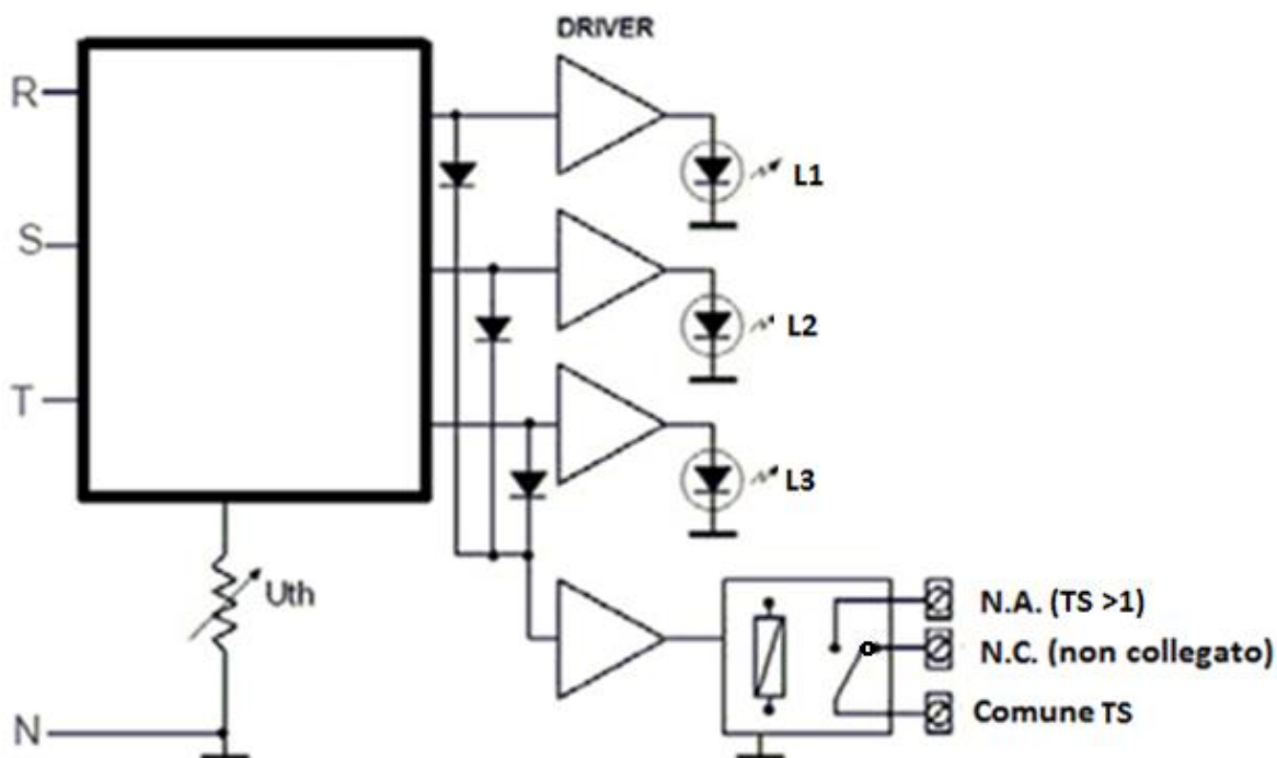
Figure 5 – Example of circuit with use of LEDs (status not activated - LEDs off)
