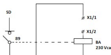
Figure 20 – Electric diagram of coil connection
