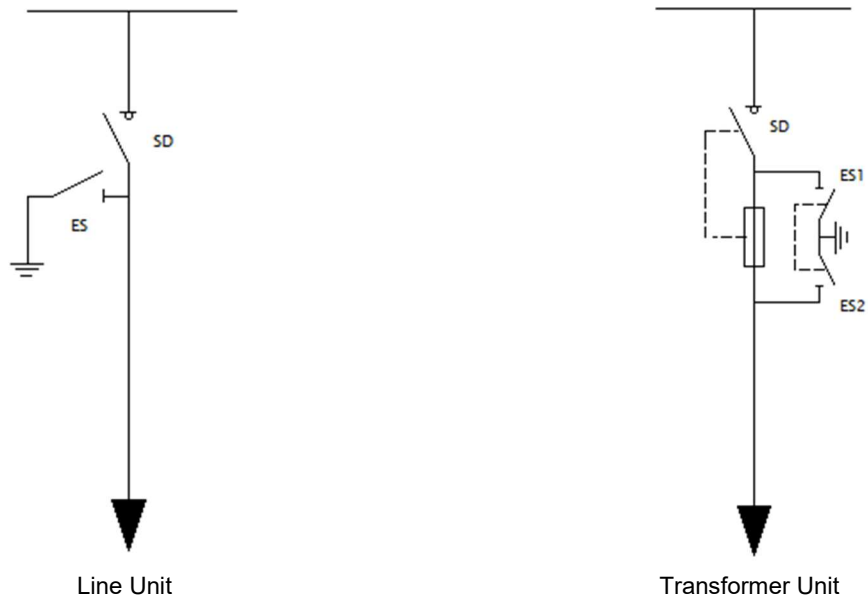
Figure 1 – Functional schemes
