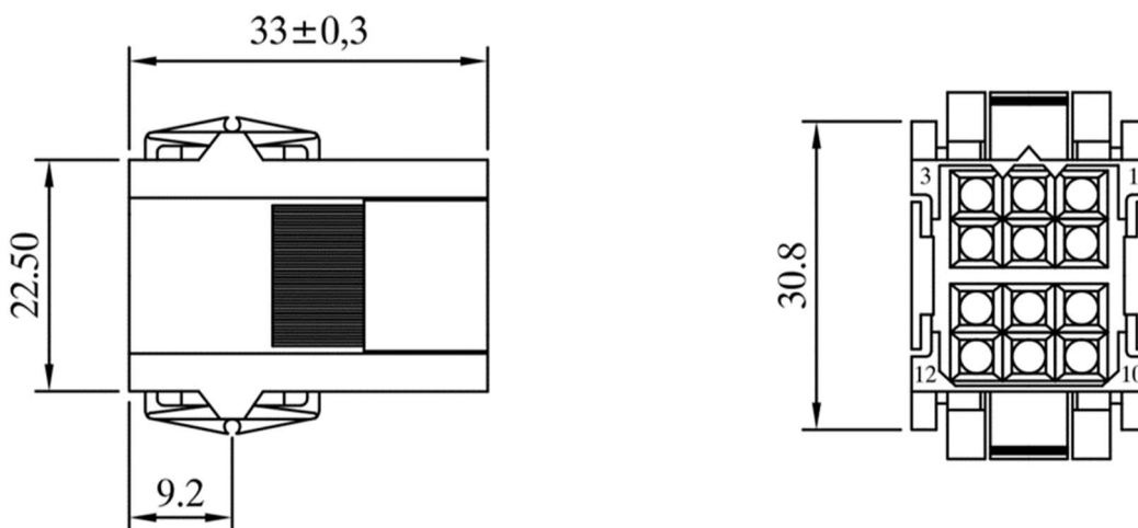
Figure 37 - Connector on the Peripheral Unit side of the cable
