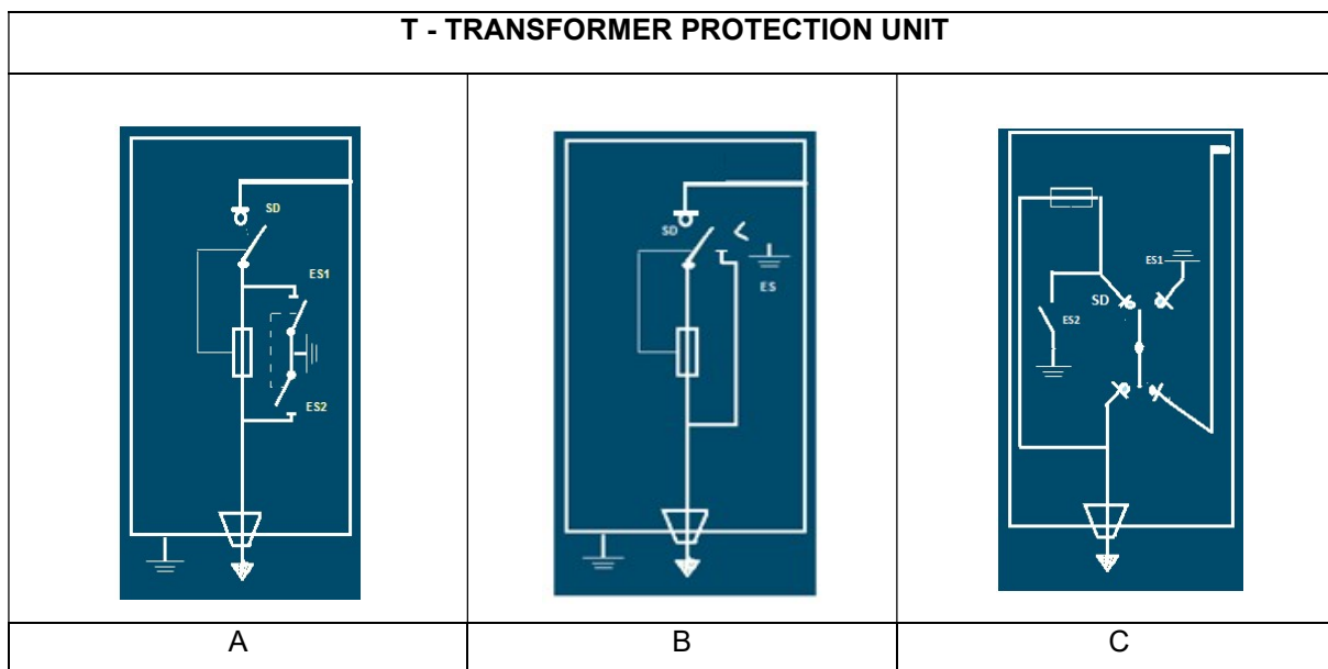
Possible constructive solutions for T unit electrical scheme
