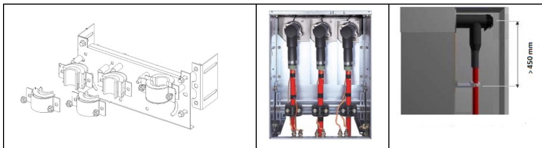
Figure 24 – Example of connectors installation
