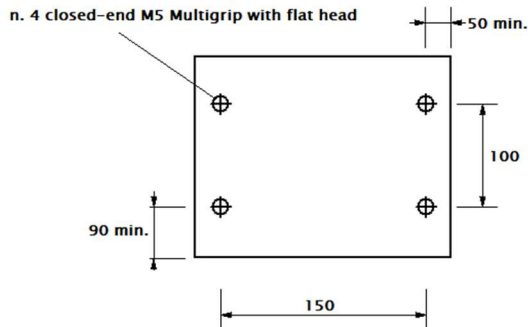
Figure 29 -Support for the fault detector device and cable duct
