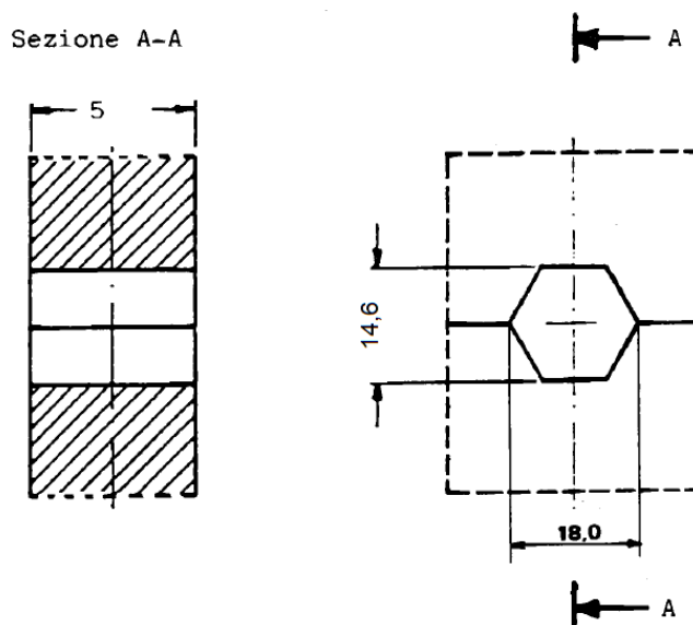
Figure 10 - hexagonal profile matrix for the contact pin lug (mm)
