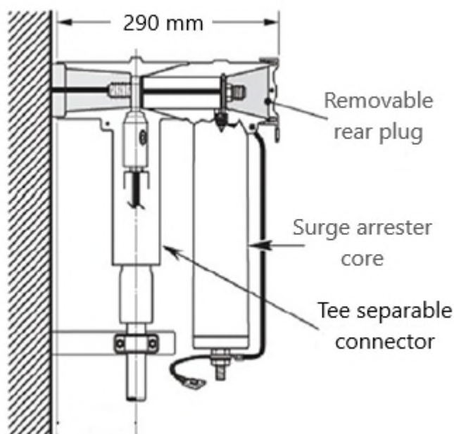
Figure 16 – Tee (asymmetric with Surge arrester) separable connector
