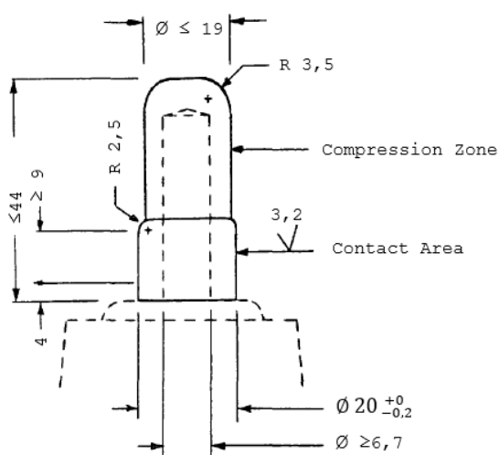
Figure 9 – Dimension of Plug contact pin for I_n=250\text{ A} (mm)
