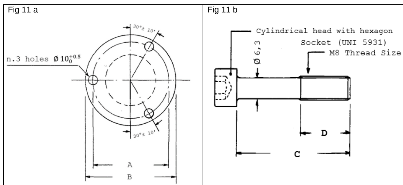
Figure 11 - Fastening device for Inner Cone separable connectors
