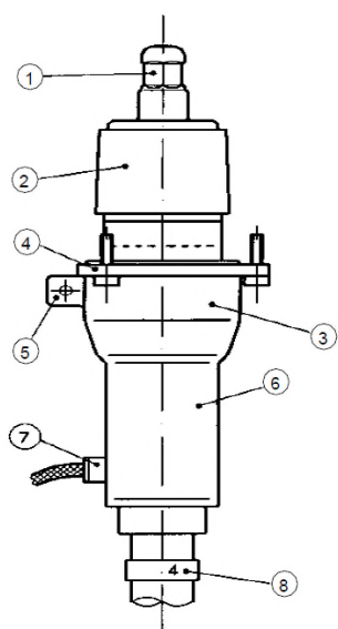
Figure 3 – Tee (symmetric with joint element) separable connector
