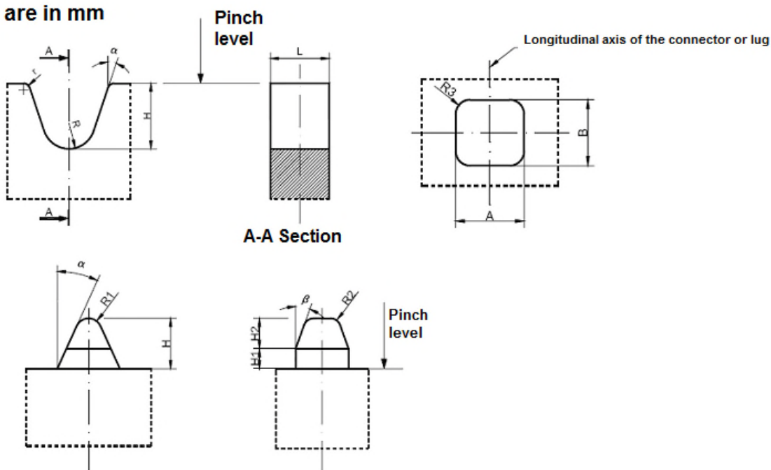
Figure 14 – Tool for compressing the earthing lug
