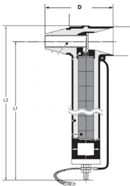
Figure 17 –Screened Surge arrester
