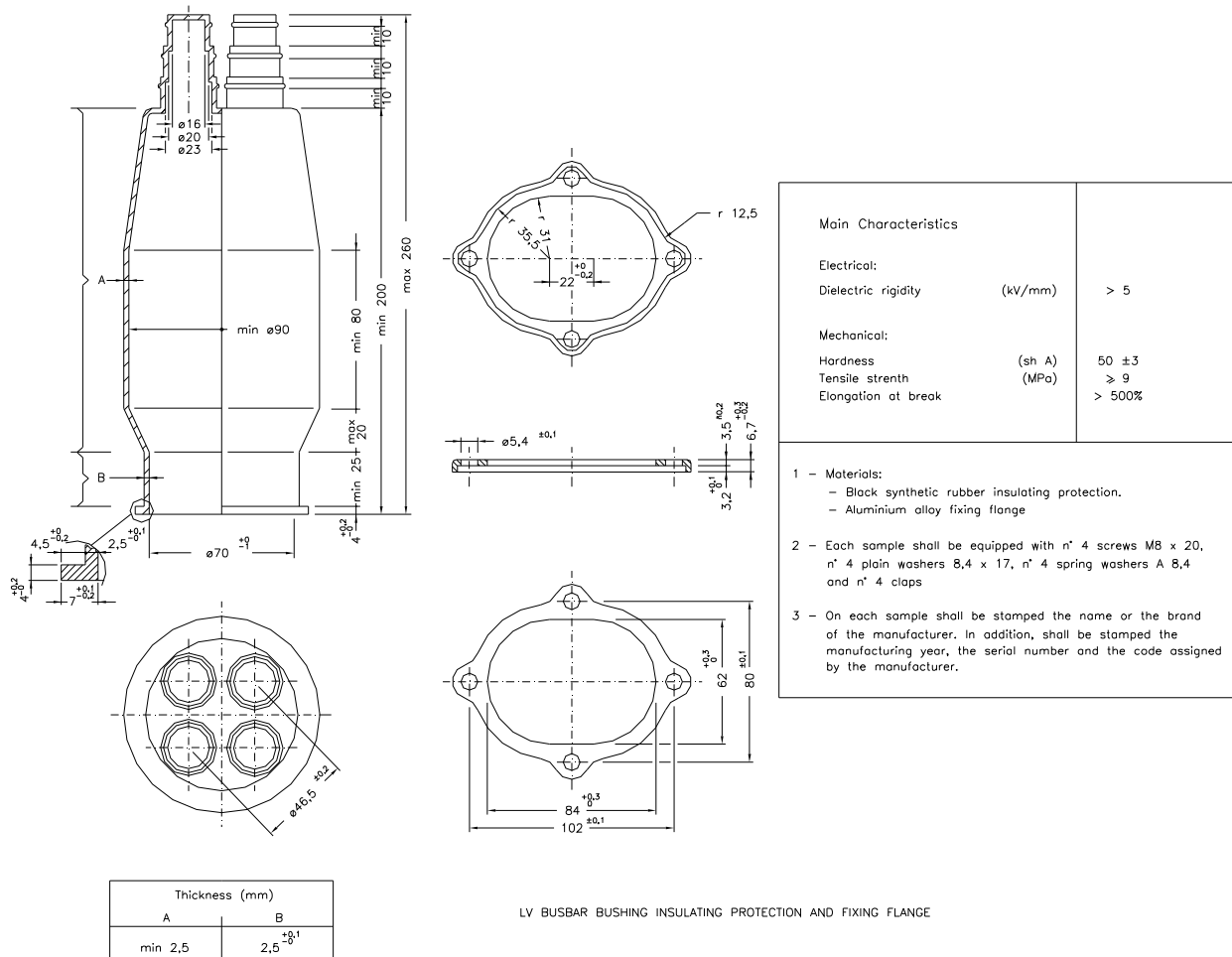
Figure C LV Bushing “Bus-bar” insulating protection
