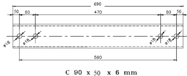
Figure A9 - Profile for anchoring base
