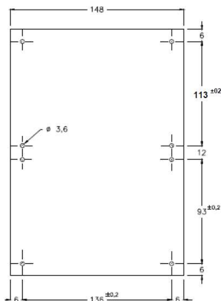
Figure C3 - Plate-holder
