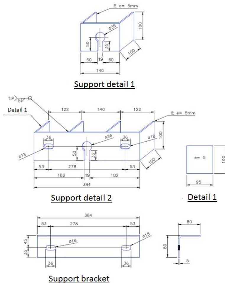
Figure A8 - Fixing support in single-pole of three-phase transformer up to 75 kVA
